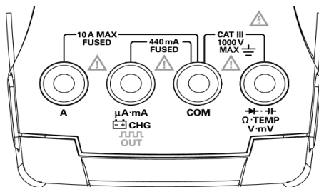
Figure 1 U1252A terminals
