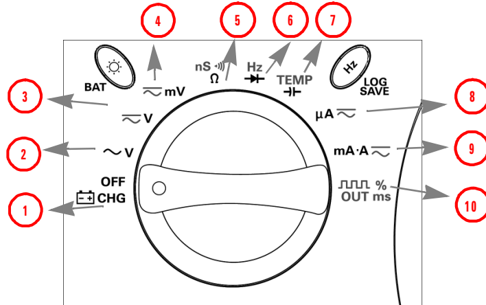
Figure 3 U1252A rotary switch
